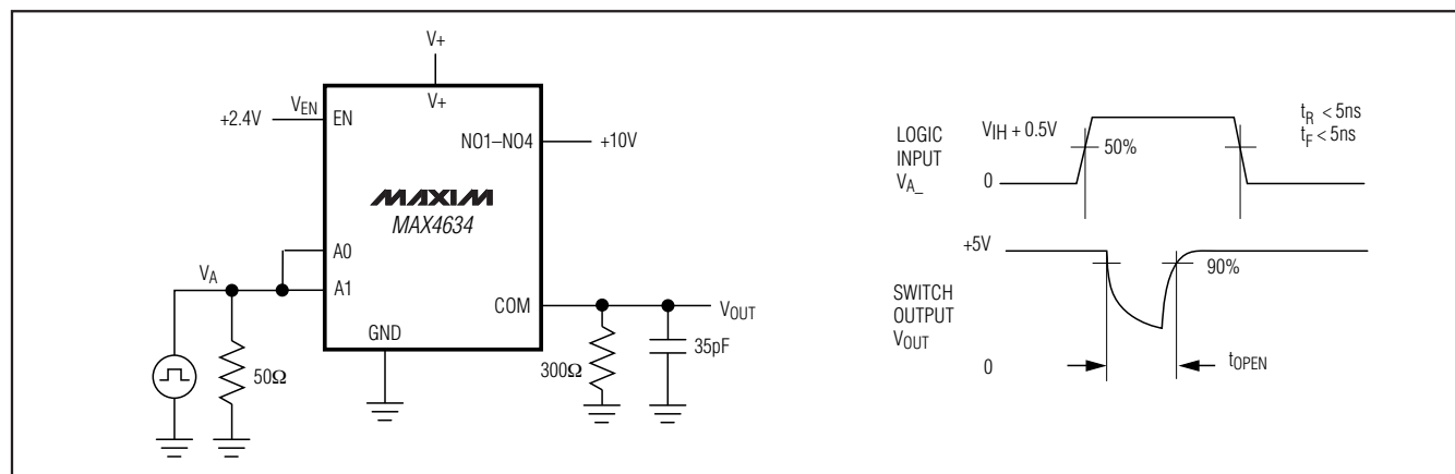
Figure 3. Break-Before-Make Interval
