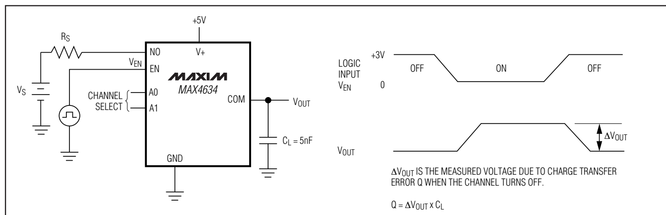
Figure 4. Charge Injection
