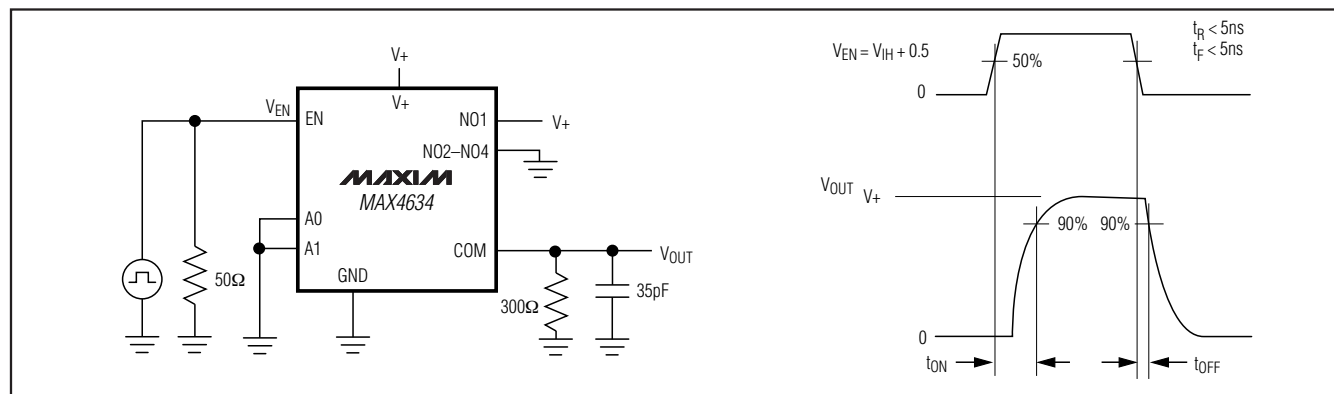
Figure 2. Switching Time
