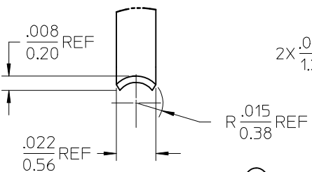
CONTACT PROFILE Detail 1 Scale 20:1
