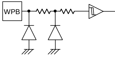
Figure 59. WPB input equivalent circuit
