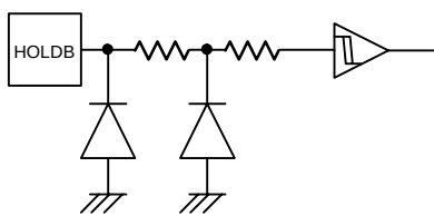
Figure 58. HOLDB input equivalent circuit
