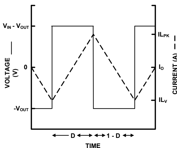
FIGURE 9. OUTPUT CURRENT
