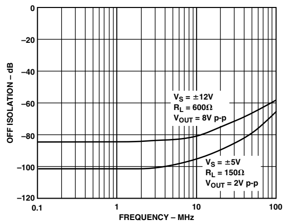
TPC 23. Off Isolation vs. Frequency
