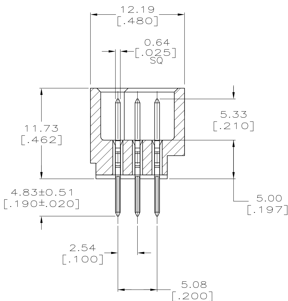
SECTION T-T
