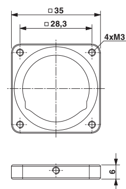
Dimensioned drawing
