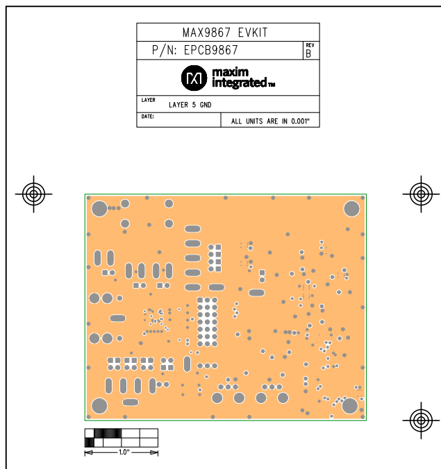
Figure 17. MAX9867 EV Kit PCB Layout—Inner Layer 5
