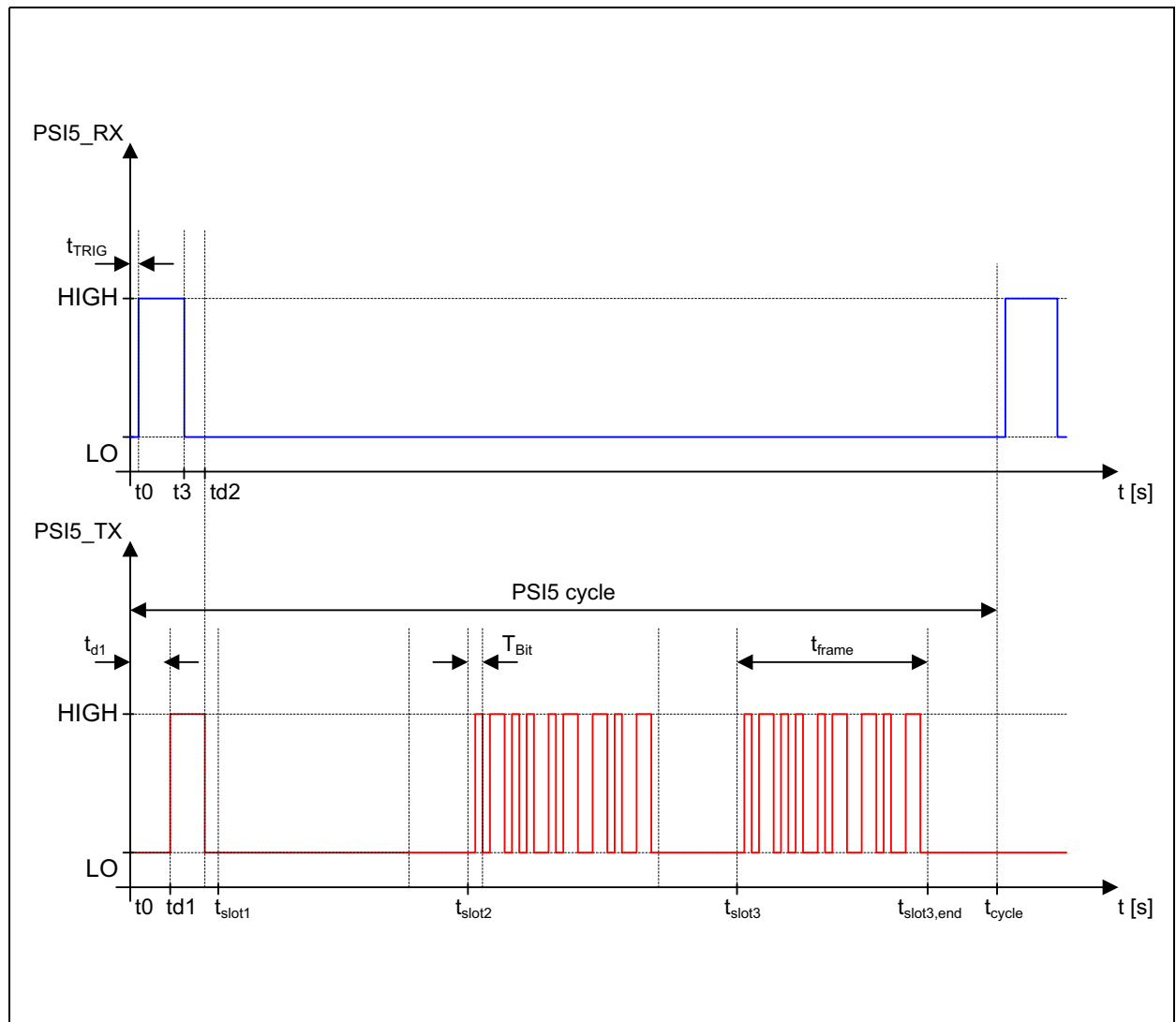
Figure 54: Synchronous Mode P10P-500/3L with Discharge Pulse
