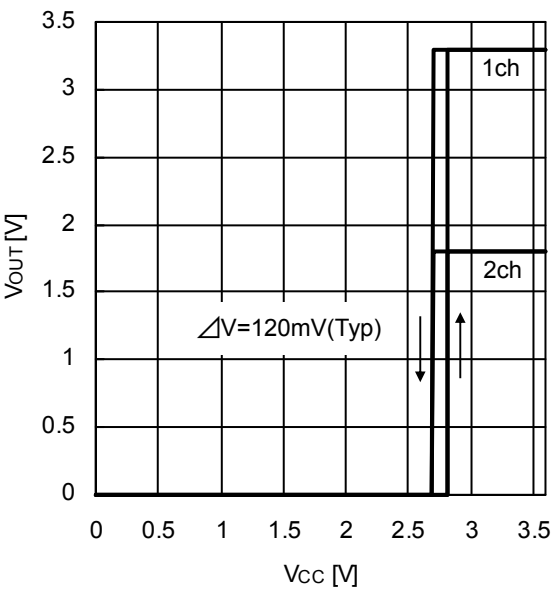
Figure.11 V cc -V out
