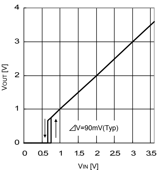
Figure.12 V in -V out
