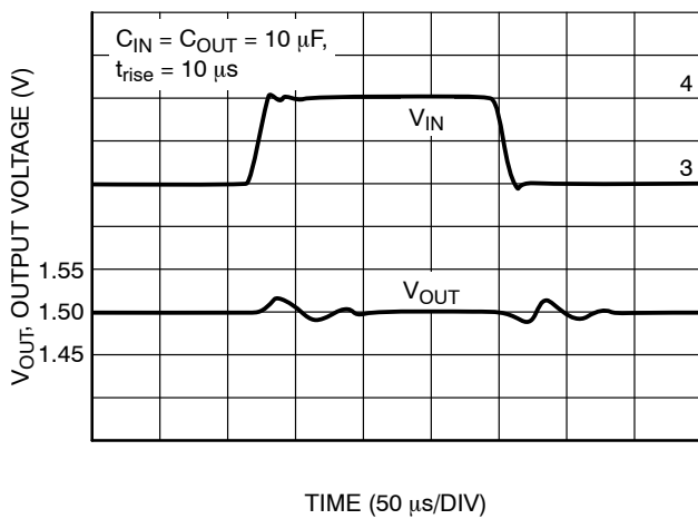
Figure 25. Line Transient ( V_{out} = 1.5 \text{ V} )
