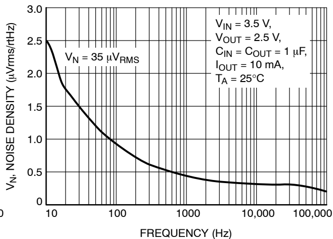
Figure 20. Noise Density vs. Frequency ( V_{out} = 2.5\text{ V} )
