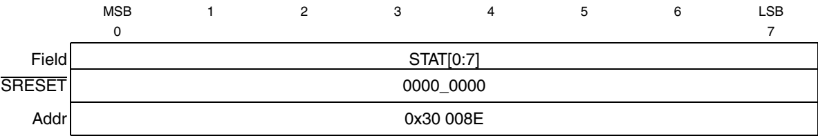
Figure 15-28. Receive Status Register (STAT)
