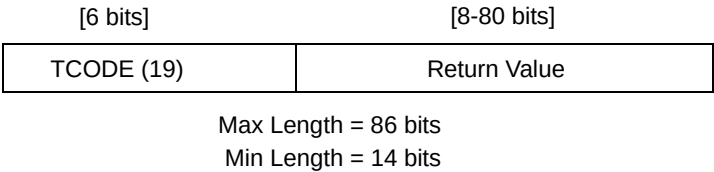
Figure 23-57. Read/Write Response Message
