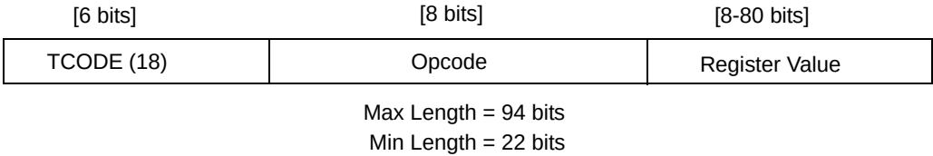
Figure 23-56. Write Register Message
