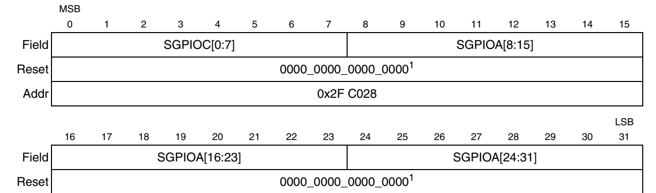
Figure 6-42. SGPIO Data Register 2 (SGPIODT2)
