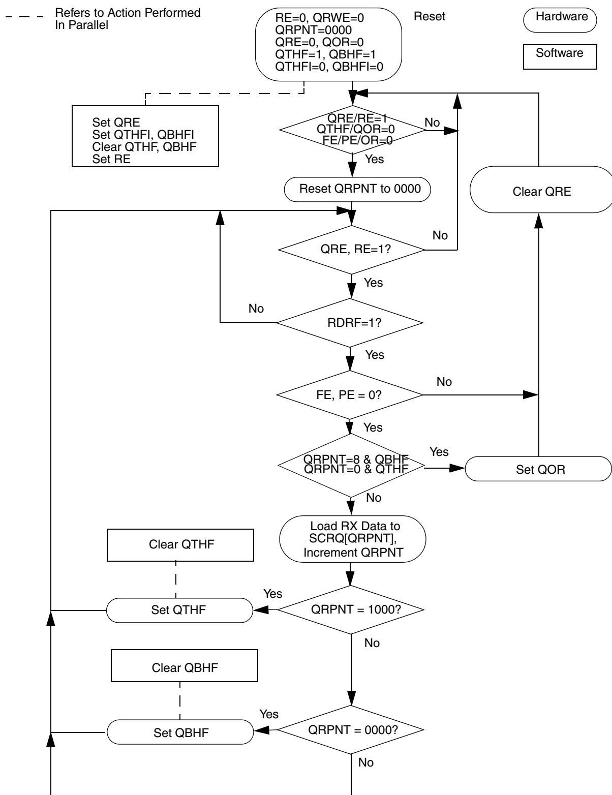
Figure 14-39. Queue Receive Flow
