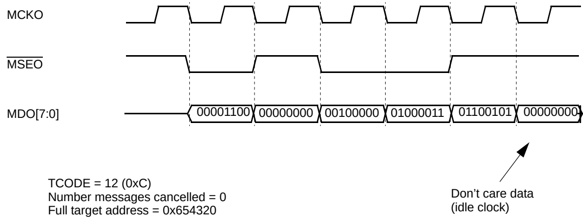
Figure 23-40. Indirect Branch Synchronization Message
