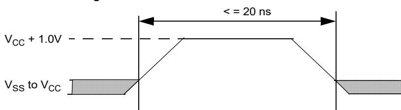
Figure 19. Maximum Positive Overshoot Waveform
