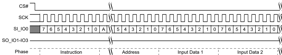
Figure 108. DYB Write Command Sequence
