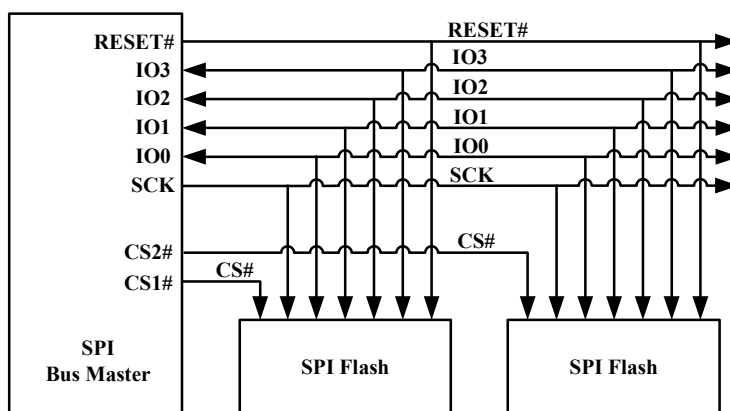
Figure 3. Bus Master and Memory Devices on the SPI Bus - Quad Bit Data Path - Separate RESET#
