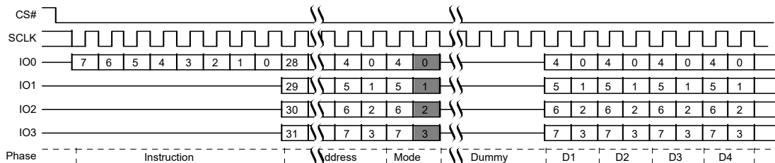
Figure 14. Quad I/O Command
