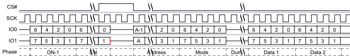
Figure 81. Dual I/O Continuous Read Command Sequence
