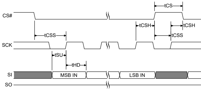
Figure 32. SPI Single Bit Input Timing
