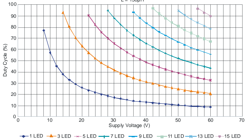
ZXLD1362 Duty Cycle L = 150\mu\text{H}
