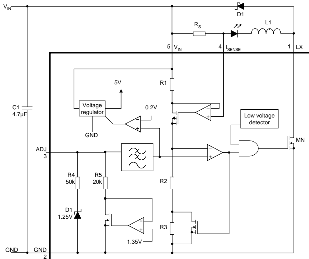
Figure 1. Block Diagram
