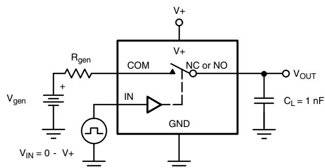
Figure 2. Charge Injection
