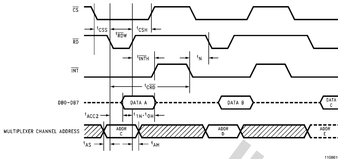
FIGURE 5. \overline{RD} Mode (Pipeline Operation) (Mode Pin is Low and t_{RDW} must be between 200 ns and 400 ns)
