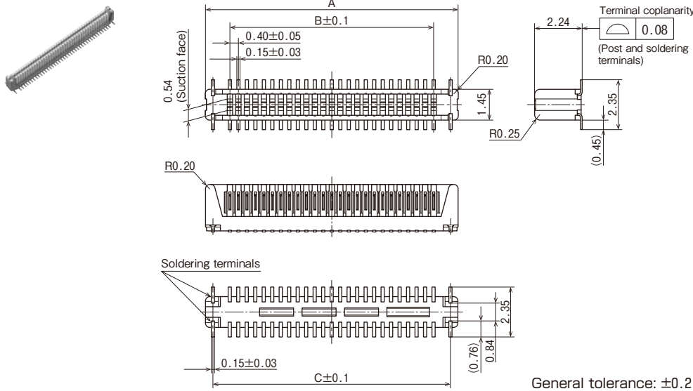
Dimension table
