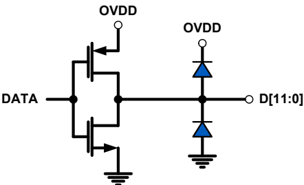
FIGURE 47. CMOS OUTPUTS
