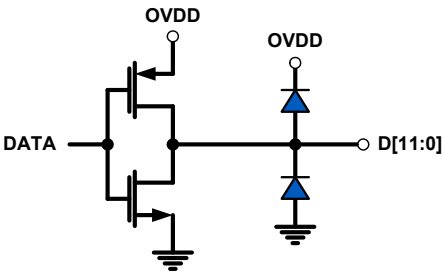
FIGURE 47. CMOS OUTPUTS
