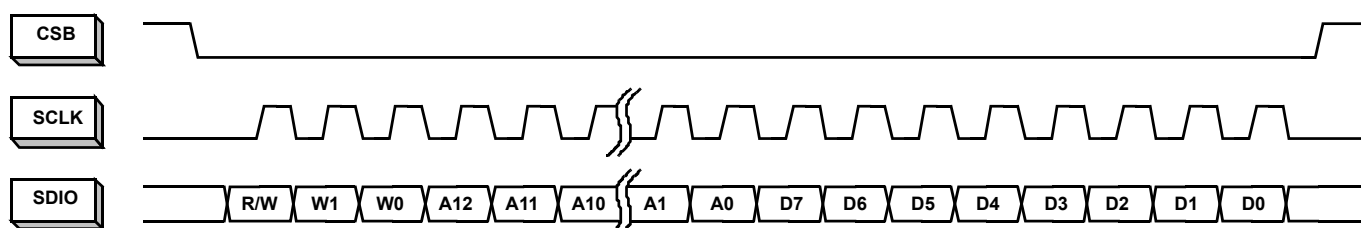
FIGURE 34. MSB-FIRST ADDRESSING
