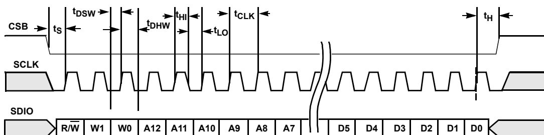
SPI WRITE
