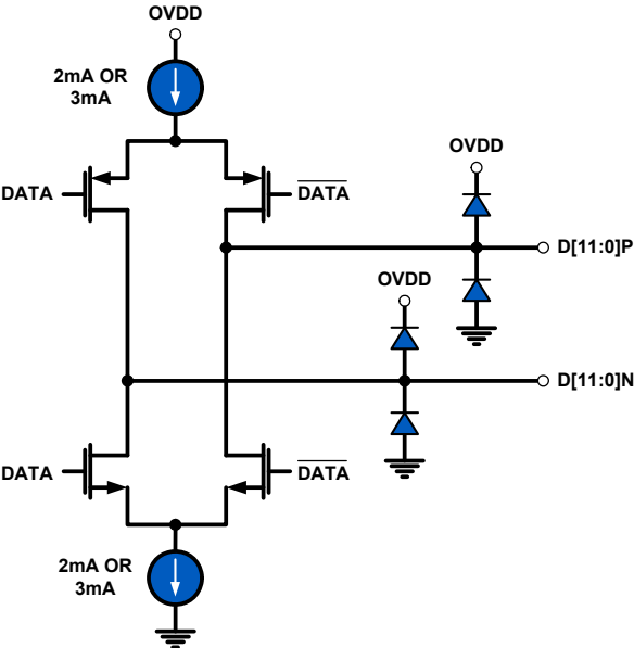
FIGURE 46. LVDS OUTPUTS
