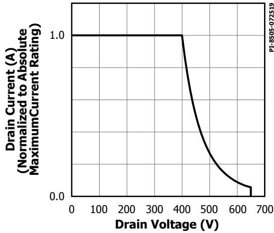
Figure 24. Maximum Allowable Drain Current vs. Drain Voltage (LYT606x).
