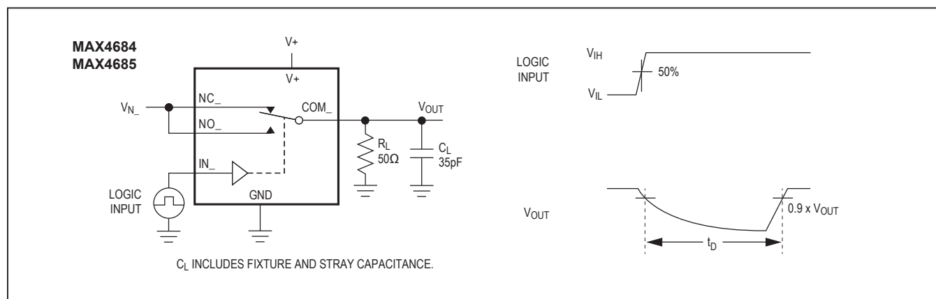
Figure 3. Break-Before-Make Interval
