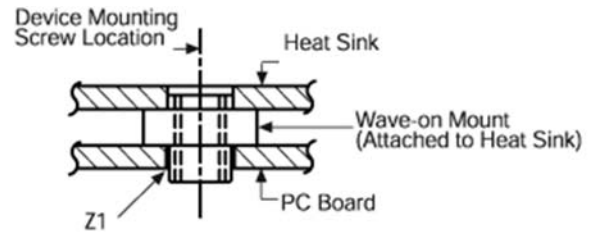
Mounting Details:
