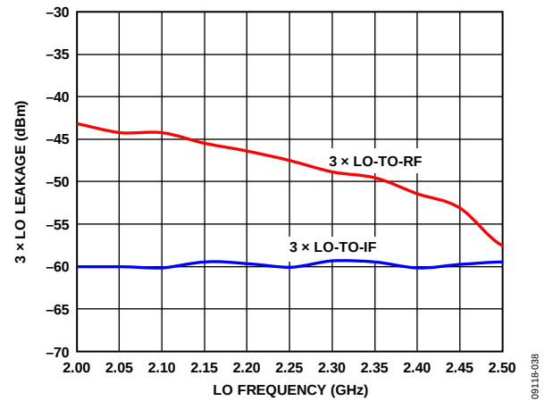
Figure 38. 3 x LO Leakage vs. LO Frequency
