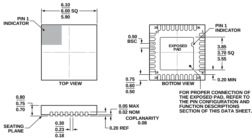
Figure 56. 36-Lead Lead Frame Chip Scale Package [LFCSP] 6 mm × 6 mm Body and 0.75 mm Package Height (CP-36-4)
