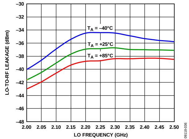
Figure 36. LO-to-RF Leakages vs. LO Frequency
