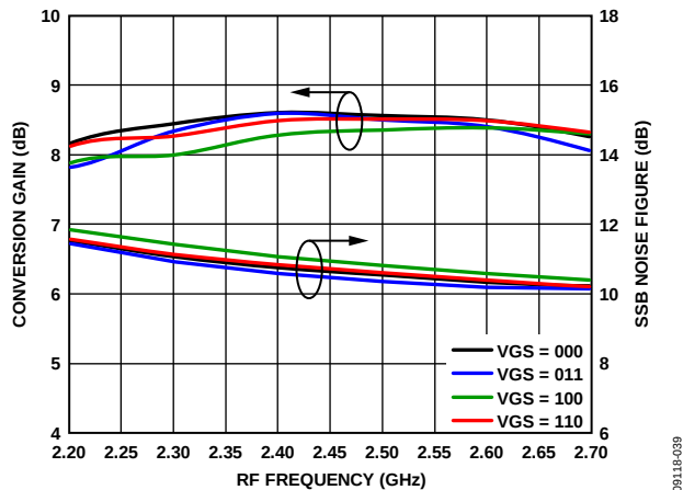
Figure 39. Power Conversion Gain and SSB Noise Figure vs. RF Frequency for Various VGS Settings
