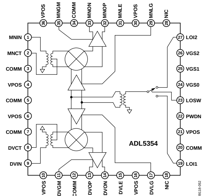
Figure 51. Simplified Schematic
