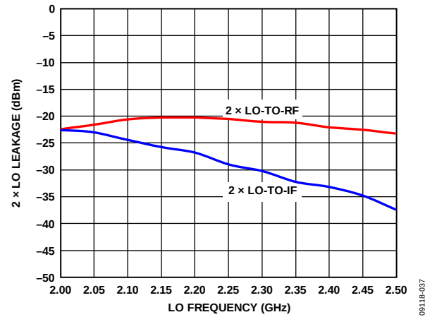
Figure 37. 2 x LO Leakage vs. LO Frequency
