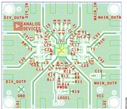
Figure 54. Evaluation Board Top Layer
