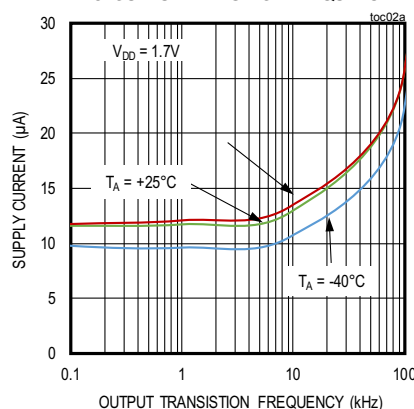
SUPPLY CURRENT vs. OUTPUT TRANSITION FREQUENCY
