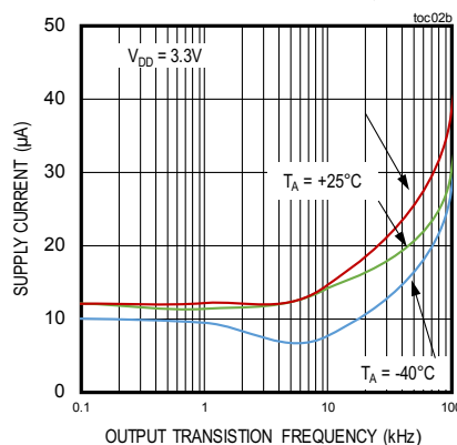
SUPPLY CURRENT vs. OUTPUT TRANSITION FREQUENCY
