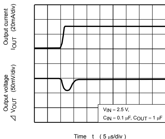
TCR5SB15 ( I_{OUT} = 1\text{m to } 30\text{mA} )
