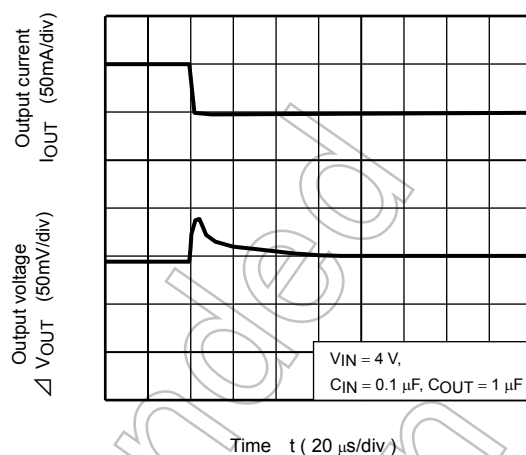
TCR5SB30 ( I_{OUT} = 100\text{m to }50\text{mA} )
