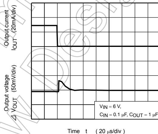
TCR5SB50 ( I_{OUT} = 30\text{m to }1\text{mA} )
