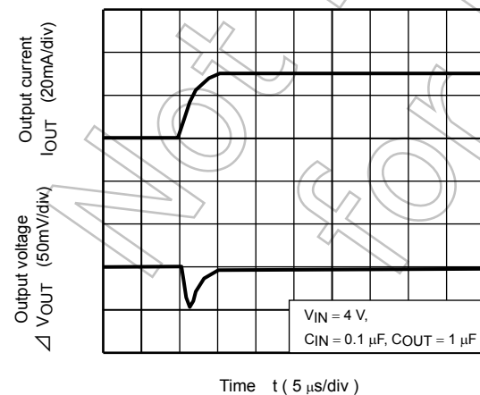
TCR5SB30 ( I_{OUT} = 1\text{m to } 30\text{mA} )
