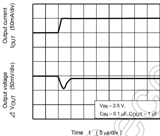
TCR5SB15 ( I_{OUT} = 50\text{m to } 100\text{mA} )
