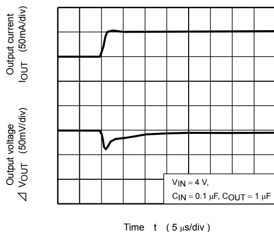
TCR5SB30 ( I_{OUT} = 50\text{m to }100\text{mA} )
