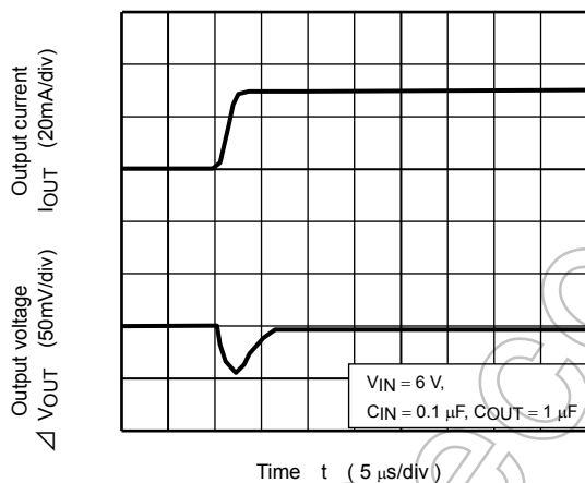
TCR5SB50 ( I_{OUT} = 1\text{m to }30\text{mA} )
