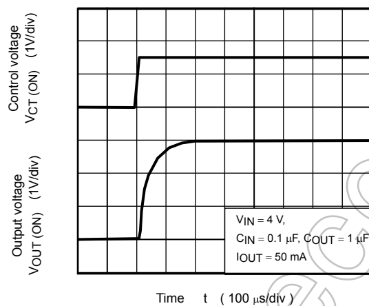
TCR5SB30 (Turn on wave form)
