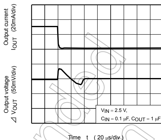
TCR5SB15 ( I_{OUT} = 30\text{m to } 1\text{mA} )
