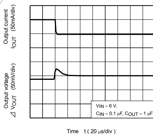
TCR5SB50 ( I_{OUT} = 100\text{m to }50\text{mA} )
