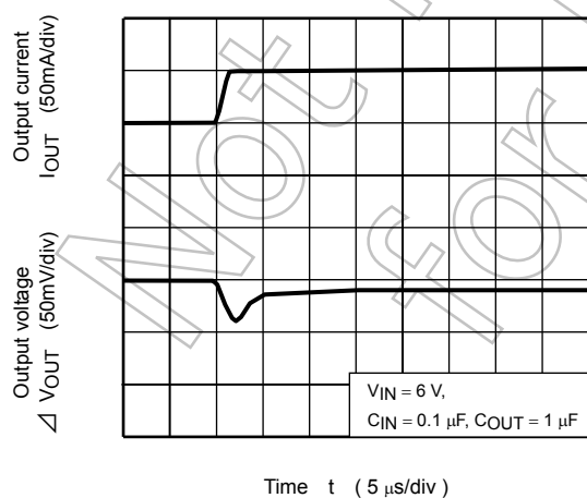
TCR5SB50 ( I_{OUT} = 50\text{m to }100\text{mA} )
