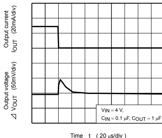
TCR5SB30 ( I_{OUT} = 30\text{m to } 1\text{mA} )
