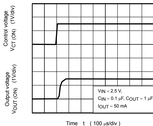
TCR5SB15 (Turn on wave form)
