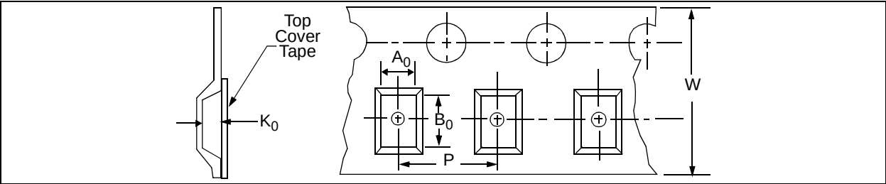
FIGURE 5-1: EMBOSSED CARRIER DIMENSIONS (8, 12, 16 AND 24 MM TAPE ONLY)
