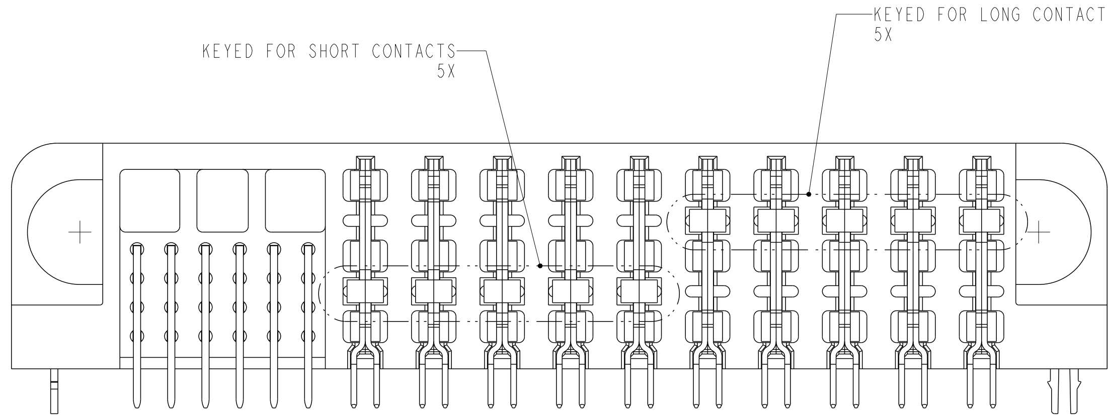
VIEW G-G
