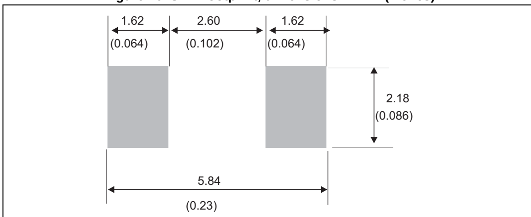
Figure 10. SMB footprint, dimensions in mm (inches)
