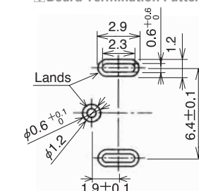
Board Termination Pattern
