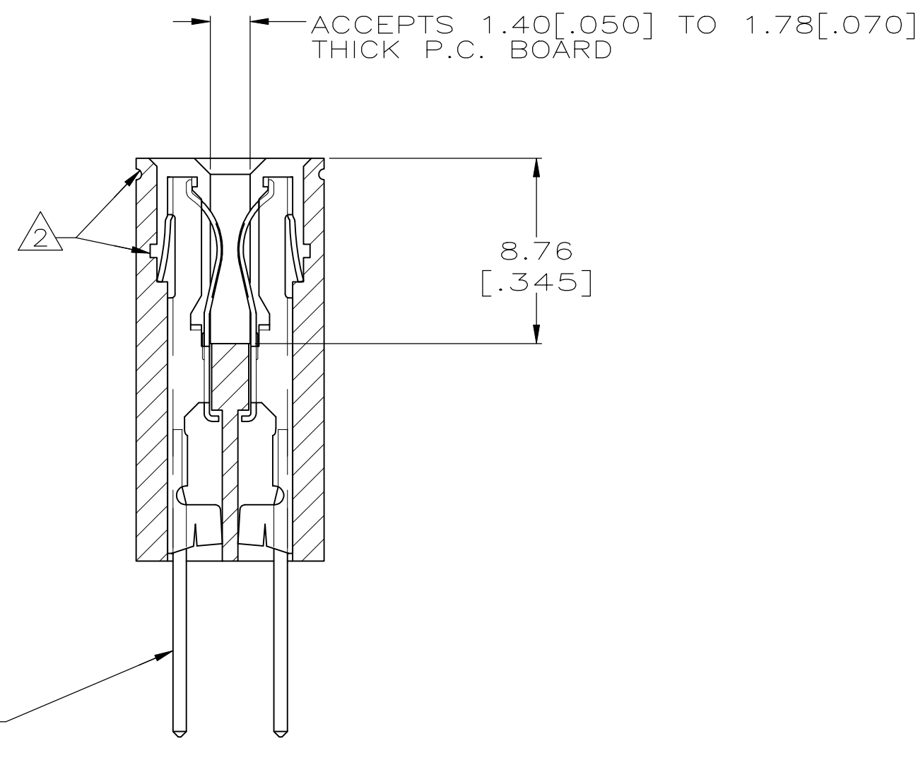
SECTION Z-Z
