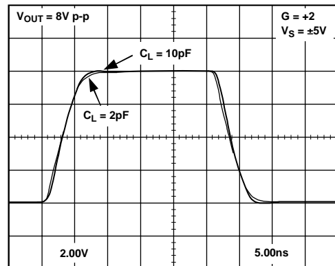
Figure 88. AD8130 Transient Response vs. Load Capacitance, V_{OUT} = 8 V p-p
