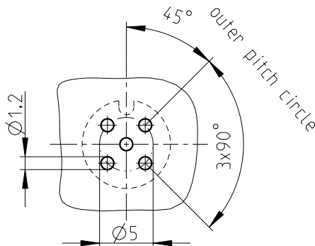
PCB-Layout (advice)
