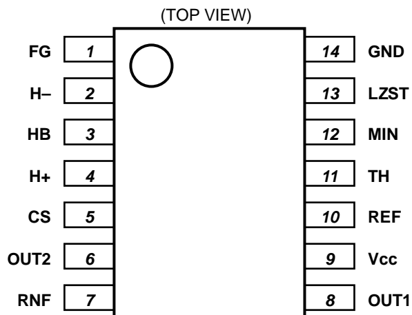
Fig.1 Pin configuration
