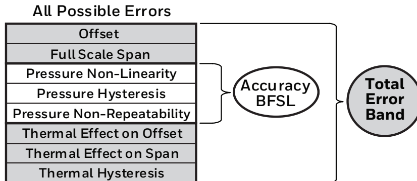
Figure 1. Total Error Band (TEB) for the Total Error Band Series
