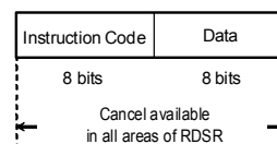
Figure 51. RDSR Cancel Valid Timing
