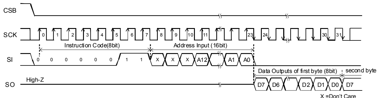
Figure 39. Read Command
