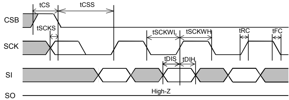
Figure 2. Input Timing
