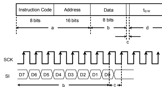
Figure 52. WRITE, WRID, LID Cancel Valid Timing
