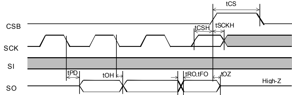
Figure 3. Input / Output Timing
