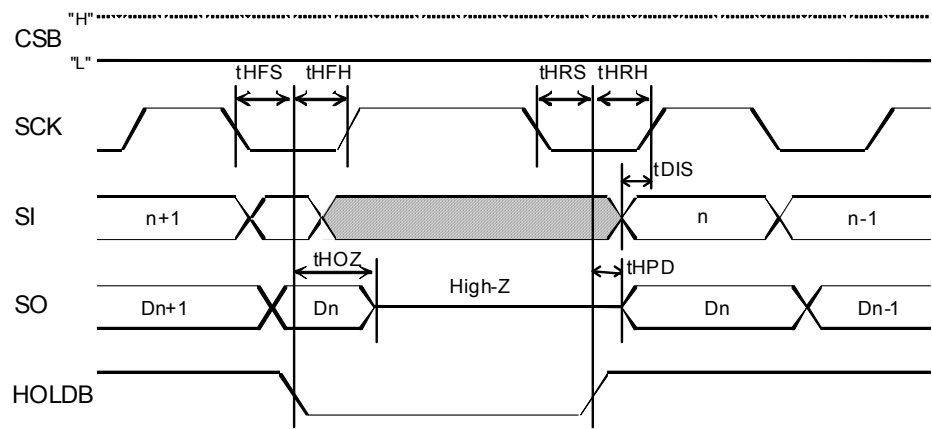
Figure 4. HOLD Timing
