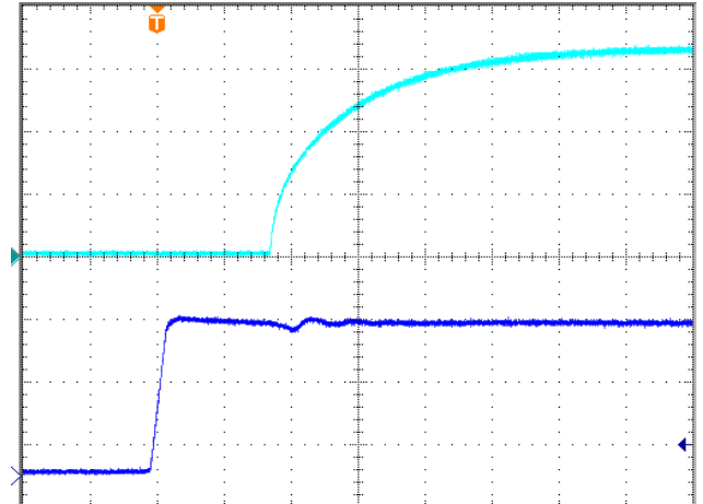
Turn-on transient at full load current (10 ms/div). Top Trace: Vout; 1.5V/div; Bottom Trace: input voltage: 10V/div.
