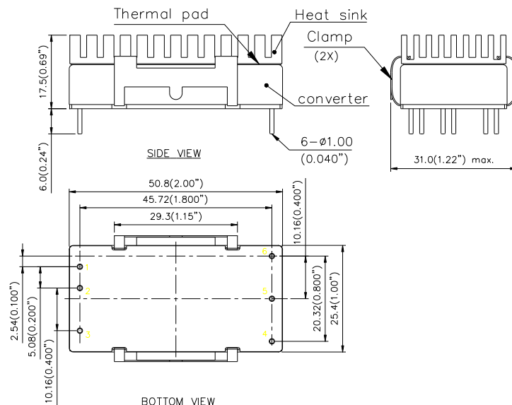
Mechanical Dimensions
