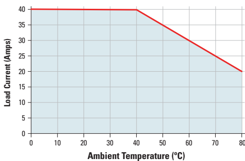
HS151DR w/50A Single or Dual SSR
