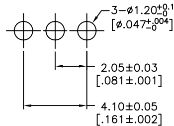
PCB MOUNTING HOLES
