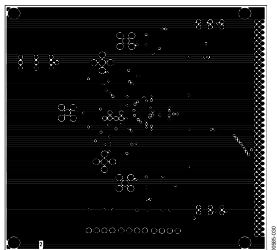
Figure 30. Ground Plane
