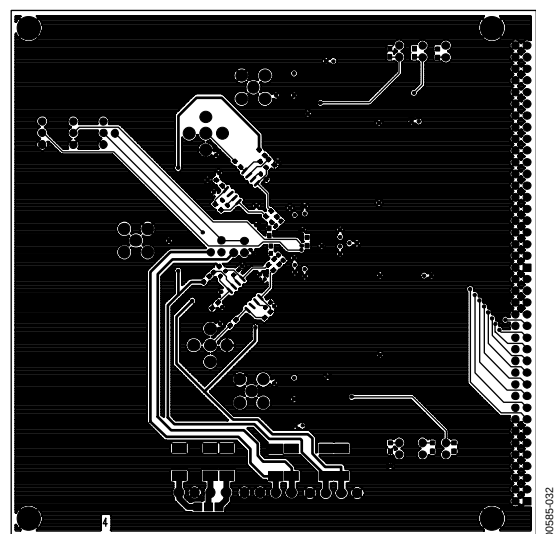
Figure 32. Bottom Routing
