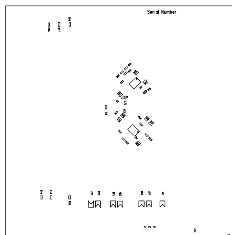
Figure 33. Bottom Silkscreen
