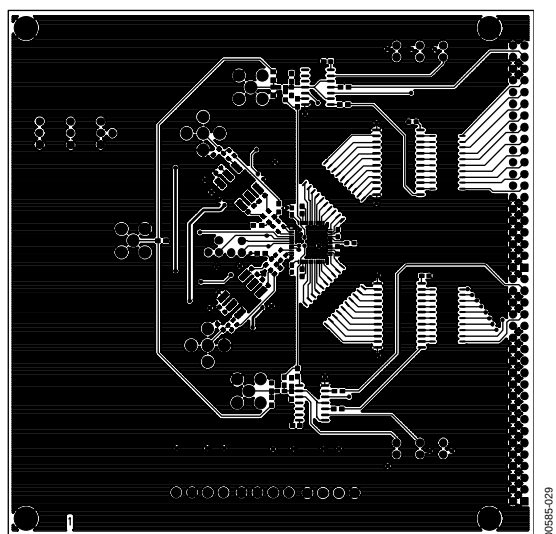
Figure 29. Top Routing
