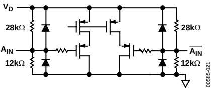
Figure 21. Equivalent Analog Input Circuit
