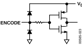
Figure 23. Equivalent Encode Input Circuit
