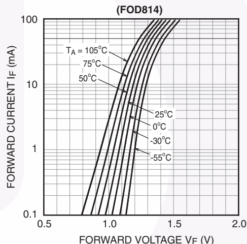
Fig. 6 Forward Current vs. Forward Voltage (FOD814)
